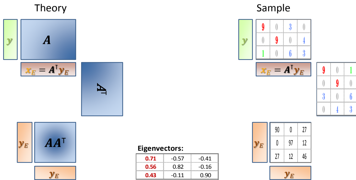
Figure 2: How the Eigenvector is calculated (Perron-Frobenius Theorem)
